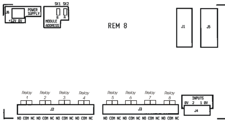
Figure 2.1 REM8 Layout Diagram
