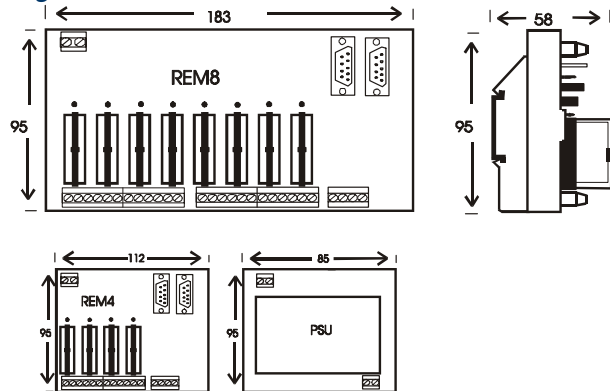
Figure 3.2 Dimensions
