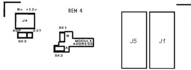
Figure 1.1 REM4 Layout Diagram
