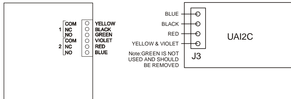
Figure 1.2 Connection Lead Details
